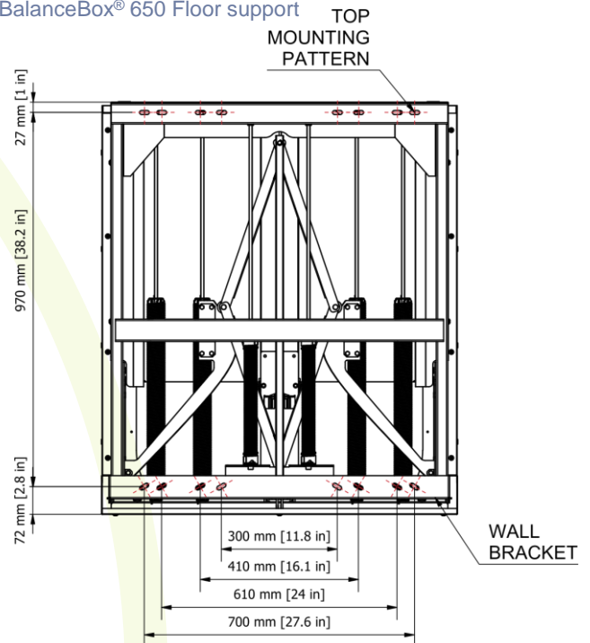
BalanceBox® 650 Wall mounting pattern (hardware for wall-mounting not included)
